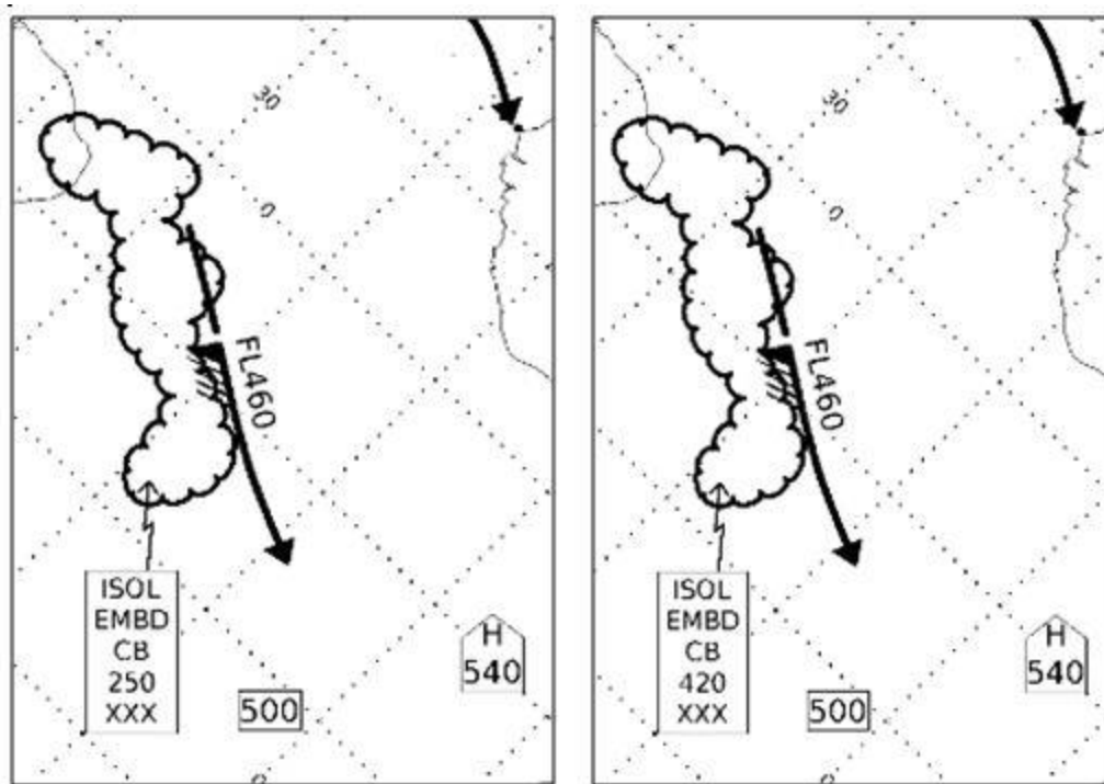
Figure 3-1 [SK28].—An example of a correction made to a SIGWX forecast issued in the PNG chart form. In the left panel, the originally issued forecast shows an erroneous height for the isolated and embedded CB cloud (FL 250) while in the right panel, the erroneous height has been replaced with the corrected value (FL 420).
