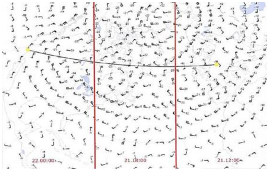
Figure 3-21. Concatenated upper wind and upper-air temperature prognostic charts based on WAFS forecasts.
